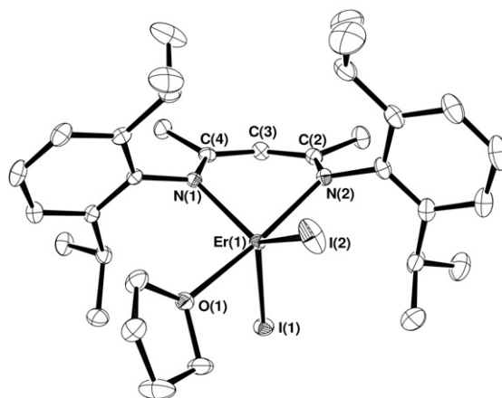
Fig. 5. ORTEP diagram (30% probability) of \text{Er}(\text{L})_2(\text{THF}) ( \text{5}\cdot\text{THF} ) with hydrogen atoms and the solvent molecule of crystallization omitted for clarity. Selected bond distances (Å) and angles ( ^\circ ): \text{Er}(1)\text{--N}(1) = 2.244(3) , \text{Er}(1)\text{--N}(2) = 2.290(3) , \text{Er}(1)\text{--I}(1) = 2.9077(5) , \text{Er}(1)\text{--I}(2) = 2.9278(4) , \text{Er}(1)\text{--O}(1) = 2.361(3) , \text{N}(1)\text{--Er}(1)\text{--N}(2) = 83.4(1) , \text{I}(1)\text{--Er}(1)\text{--I}(2) = 132.24(1) , \text{I}(1)\text{--Er}(1)\text{--N}(1) = 101.30(7) , \text{I}(2)\text{--Er}(1)\text{--N}(1) = 126.14(7) , \text{O}(1)\text{--Er}(1)\text{--N}(2) = 168.4(1) .
