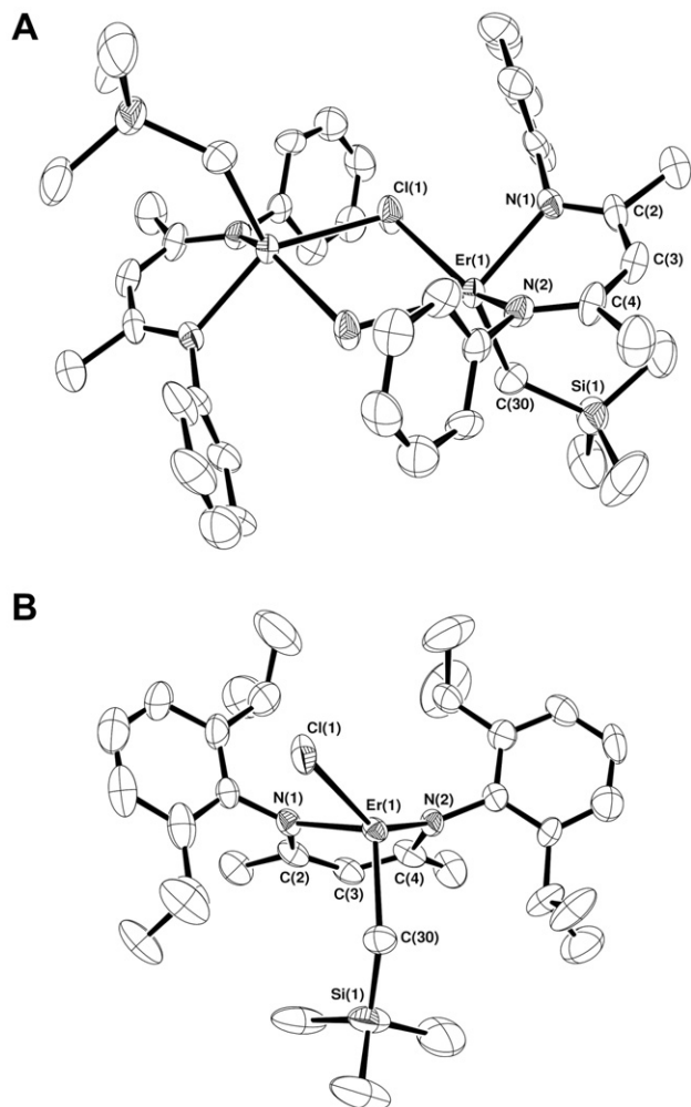
Fig. 3. ORTEP diagram (50% probability) of [\text{Er}(\text{L})(\text{CH}_2\text{SiMe}_3)(\mu\text{-Cl})]_2 ( 3 ). The dimeric structure (with hydrogen atoms and ^1\text{Pr} groups omitted for clarity) is shown in (A), while the asymmetric unit (with hydrogen atoms omitted for clarity) is depicted in (B). Selected bond distances (Å) and angles ( ^\circ ): \text{Er}(1)\text{-N}(1) = 2.284(5) , \text{Er}(1)\text{-N}(2) = 2.270(5) , \text{Er}(1)\text{-Cl}(1) = 2.653(2) , \text{Er}(1)\text{-Cl}(1)_1 = 2.638(2) , \text{Er}(1)\text{-C}(30) = 2.343(7) , \text{N}(1)\text{-Er}(1)\text{-N}(2) = 85.4(2) , \text{Cl}(1)\text{-Er}(1)\text{-Cl}(1)_1 = 77.4(1) , \text{Cl}(1)\text{-Er}(1)\text{-N}(2) = 142.2(2) , \text{Cl}(1)\text{-Er}(1)\text{-N}(1) = 86.3(2) , \text{Cl}(1)_1\text{-Er}(1)\text{-N}(2) = 87.9(1) , \text{Cl}(1)_1\text{-Er}(1)\text{-N}(1) = 143.5(1) , \text{C}(30)\text{-Er}(1)\text{-N}(1) = 107.9(2) , \text{C}(30)\text{-Er}(1)\text{-N}(2) = 109.5(2) , \text{C}(30)\text{-Er}(1)\text{-Cl}(1) = 108.2(2) , \text{C}(30)\text{-Er}(1)\text{-Cl}(1)_1 = 108.2(2) . Note: \text{Cl}(1)_1 was generated by the symmetry operator -x+2, -y+1, -z+2 .
