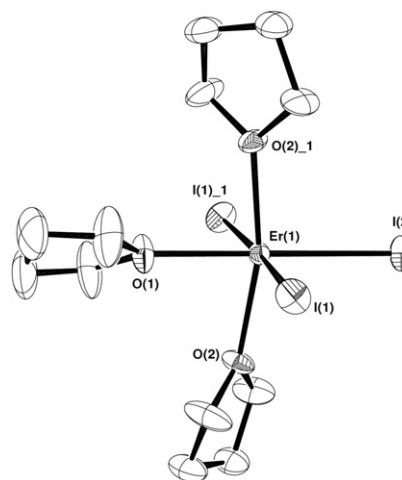
Fig. 6. ORTEP diagram (50% probability) of \text{ErI}_3(\text{THF})_3 ( 6 ). Selected bond distances (Å) and angles ( ^\circ ): \text{Er}(1)\text{--I}(2) = 2.9276(6) , \text{Er}(1)\text{--I}(1) = 2.9504(4) , \text{Er}(1)\text{--O}(1) = 2.327(5) , \text{Er}(1)\text{--O}(2) = 2.273(3) , \text{I}(2)\text{--Er}(1)\text{--I}(1) = 91.99(1) , \text{I}(1)\text{--Er}(1)\text{--O}(1) = 88.01(1) , \text{I}(2)\text{--Er}(1)\text{--O}(2) = 97.03(9) , \text{I}(1)\text{--Er}(1)\text{--O}(2) = 90.18(9) , \text{O}(2)\text{--Er}(1)\text{--O}(1) = 82.97(9) . Note: \text{I}(1)_1 and \text{O}(2)_1 were generated by the symmetry operator -x + 1, y, -z + 0.5 .
