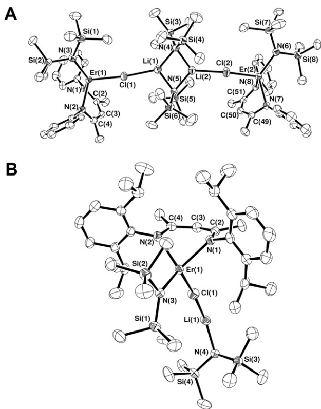
Fig. 2. ORTEP diagram (50% probability) of [\text{Er}(\text{L})\text{N}(\text{SiMe}_3)_2\text{Cl}(\mu\text{-LiN}(\text{SiMe}_3)_2)]_2 ( 2 ). The dimeric structure (with hydrogen atoms and ^i\text{Pr} groups omitted for clarity) is shown in (A), while a monomeric moiety (with hydrogen atoms omitted for clarity) is depicted in (B). Selected bond distances (Å) and angles ( ^\circ ): Er(1)–N(1) = 2.259(3), Er(1)–N(2) = 2.256(3), Er(1)–N(3) = 2.193(3), Er(1)–Cl(1) = 2.5382(9), Er(2)–N(6) = 2.198(3), Er(2)–N(7) = 2.261(3), Er(2)–N(8) = 2.248(3), Er(2)–Cl(2) = 2.533(1), Li(1)–Cl(1) = 2.499(6), Li(2)–Cl(2) = 2.492(6), Li(1)–N(5) = 2.005(7), Li(2)–N(5) = 2.013(7), Li(1)–N(4) = 2.034(7), Li(2)–N(4) = 2.024(7), N(1)–Er(1)–N(2) = 84.3(1), N(1)–Er(1)–Cl(1) = 105.71(7), N(1)–Er(1)–N(3) = 124.8(1), N(2)–Er(1)–Cl(1) = 106.91(8), N(2)–Er(1)–N(3) = 116.3(1), N(3)–Er(1)–Cl(1) = 114.31(8), N(8)–Er(2)–N(7) = 87.1(1), N(7)–Er(2)–Cl(2) = 104.35(8), N(7)–Er(2)–N(6) = 125.5(1), N(8)–Er(2)–Cl(2) = 107.86(8), N(8)–Er(2)–N(6) = 114.4(1), N(6)–Er(2)–Cl(2) = 113.93(8), Li(1)–N(5)–Li(2) = 75.7(3), Li(1)–N(4)–Li(2) = 74.9(3), N(5)–Li(1)–N(4) = 104.7(3), N(5)–Li(2)–N(4) = 104.8(3).
